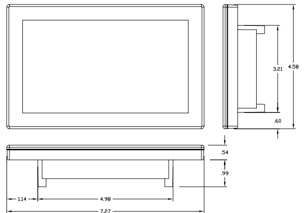
ST3+™ Dimensions
